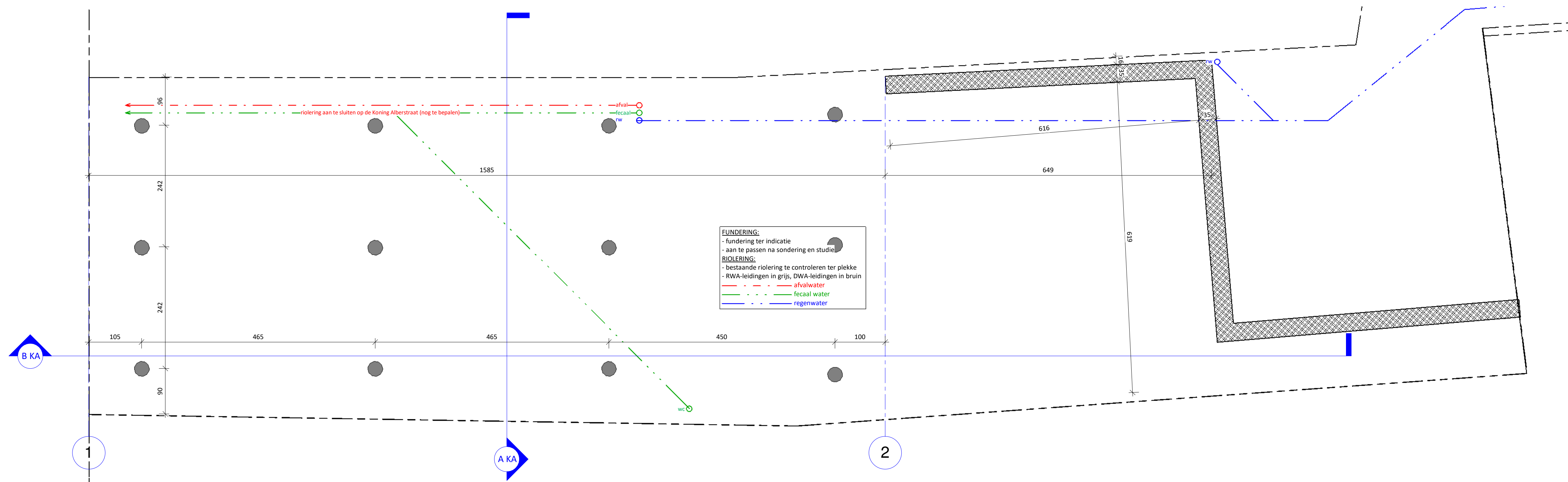
1 FUNDERING/RIOLERING 1 : 50
