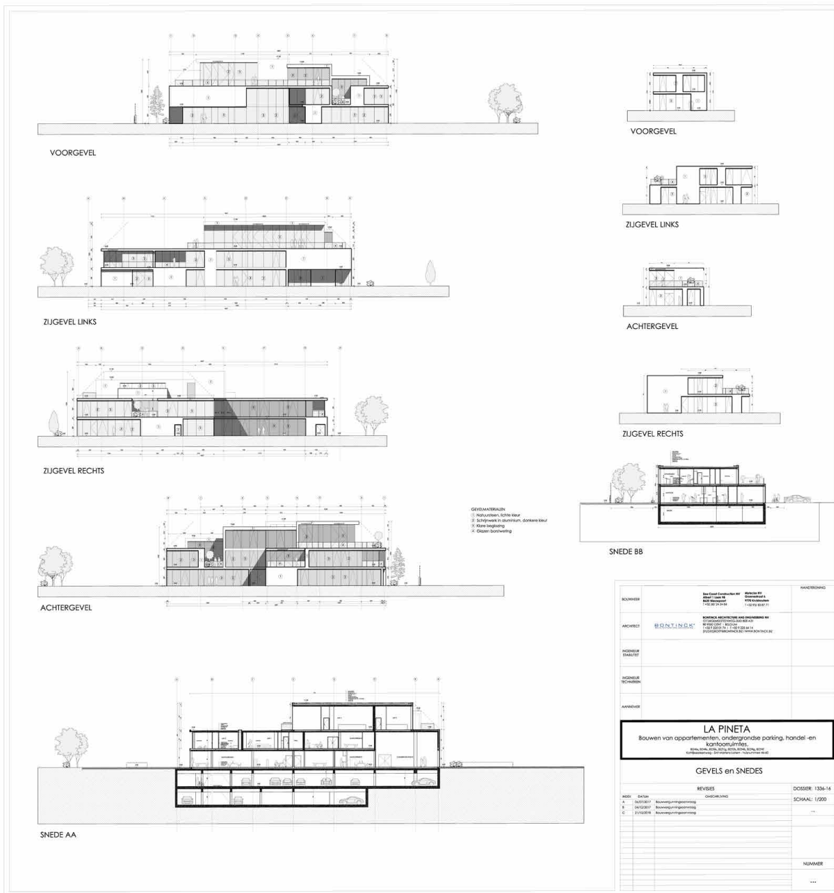
Figuur 33: Doorsnedes (© Bontinck Architecture & Engineering NV)
