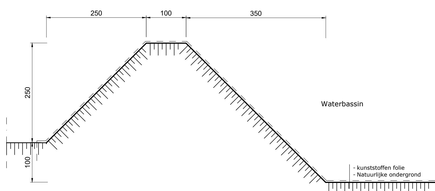
- principe waterbassin 1/50 -
