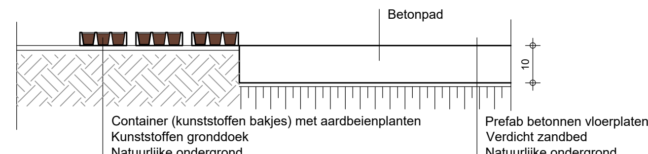
- principedetail betonpad/trayveld 1/20 -
