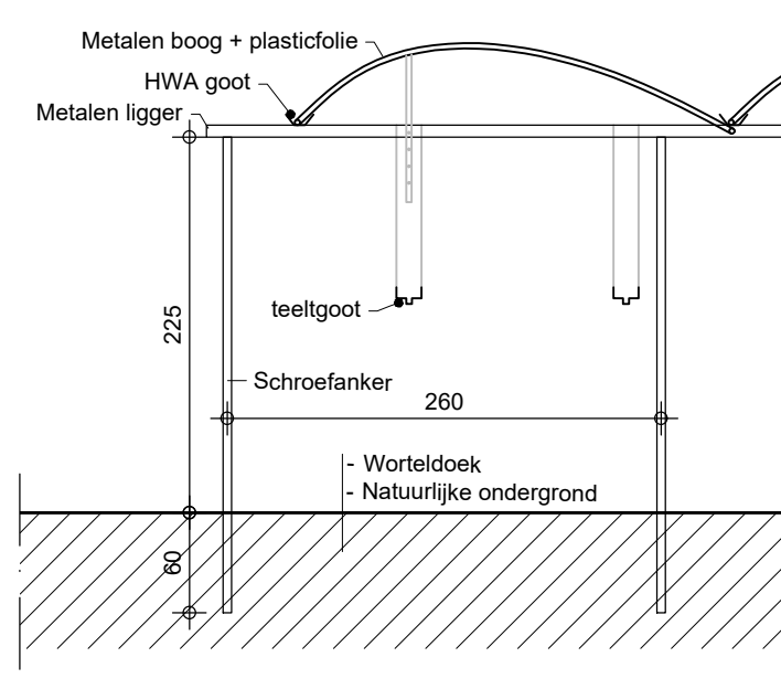
- principe plastic tunnels 1/50 -
