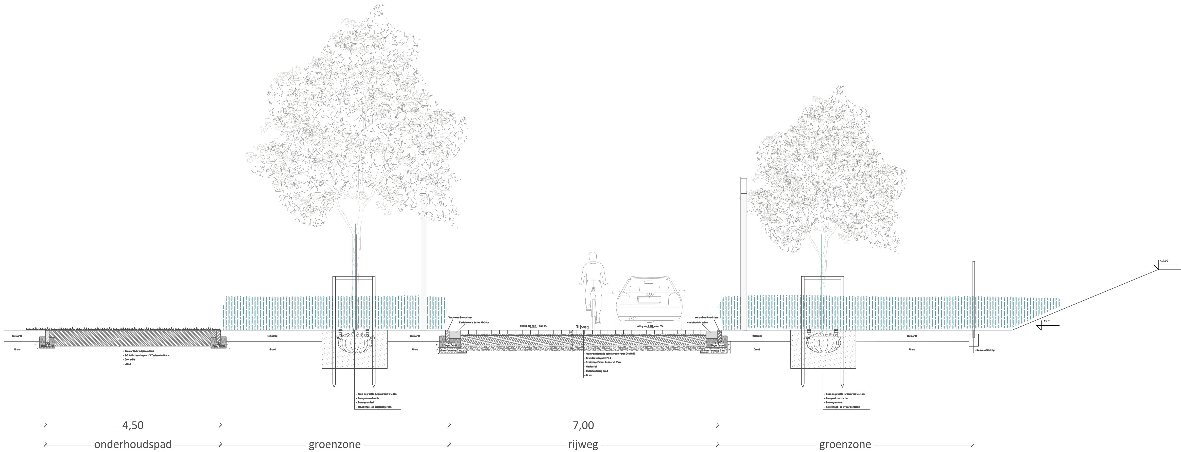
| PROFIEL AA' |
