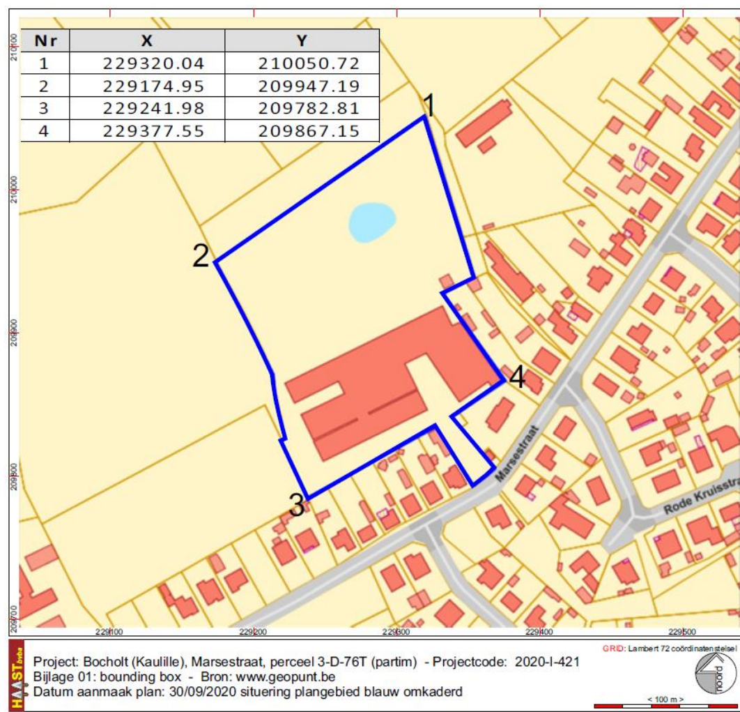
Fig. 1: Bounding Box
