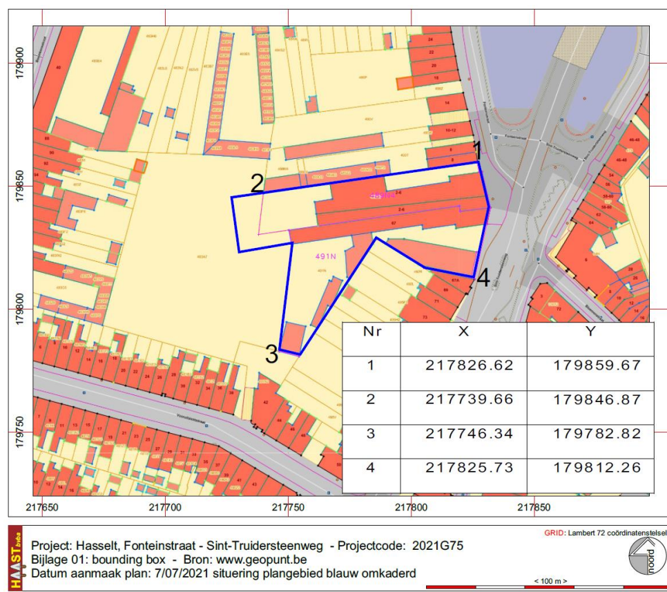
Fig. 1: Bounding Box
