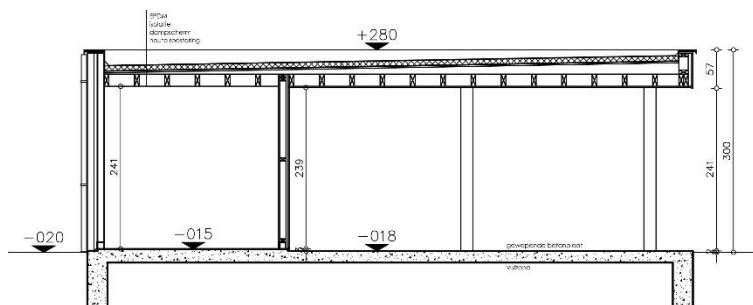
DOORSNEDE HH carports 7 tem 12 SCHAAL 1/50
