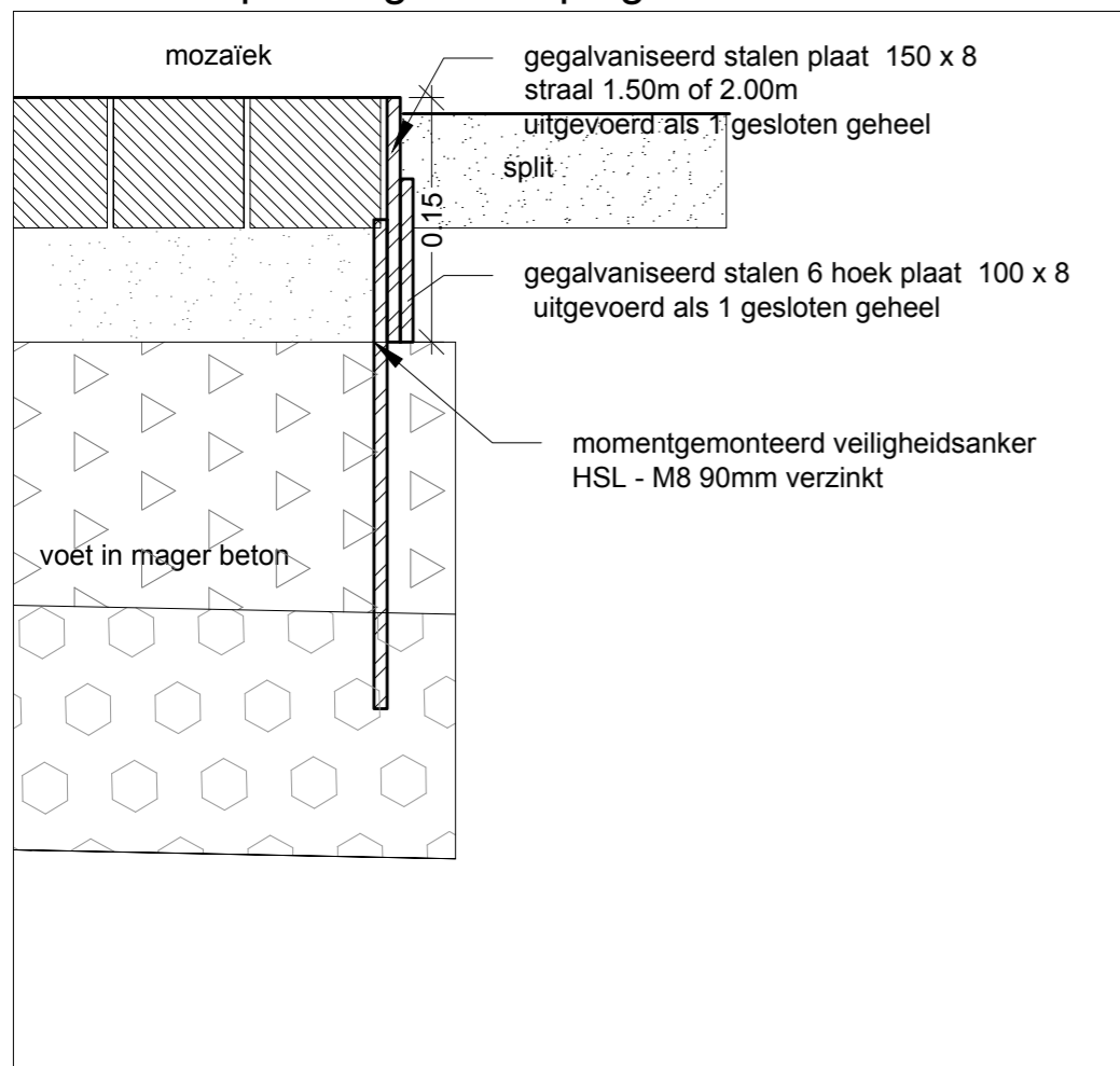
detail C: opsluiting boomspiegel 1/5
