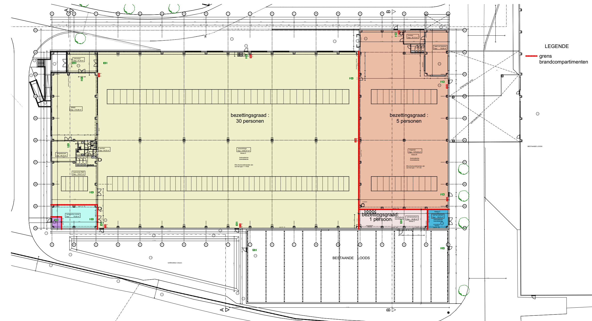
BRANDCOMPARTIMENTEN 1/500
