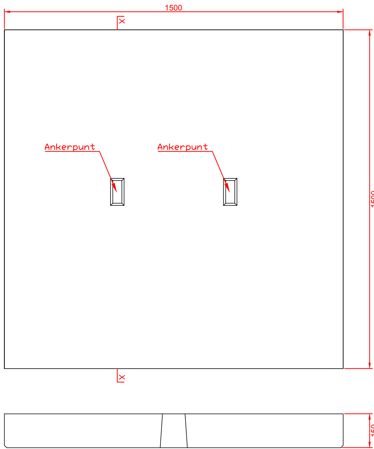
Detail betonplaten
