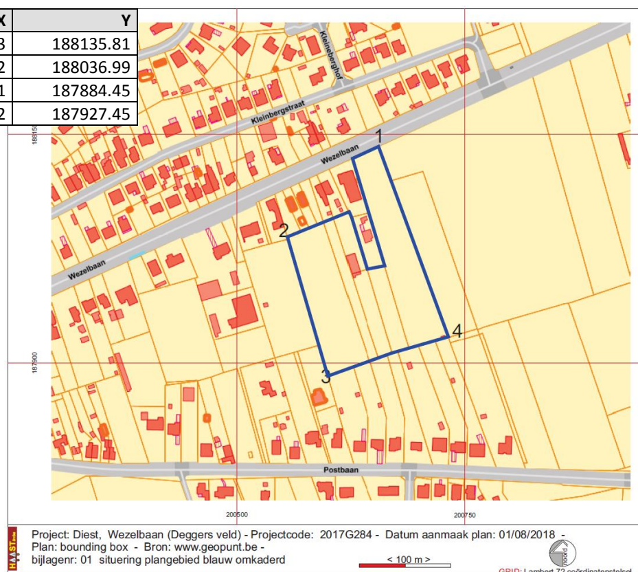
Fig. 1: Bounding Box
